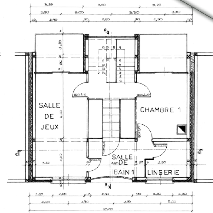
PLAN R+1
